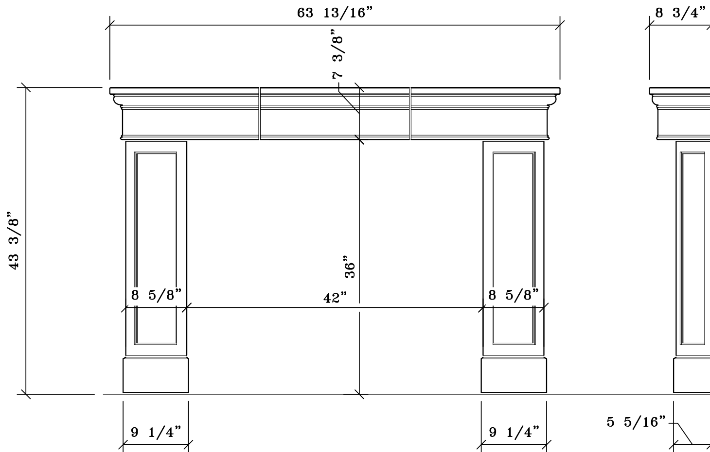
FRONT VIEW
