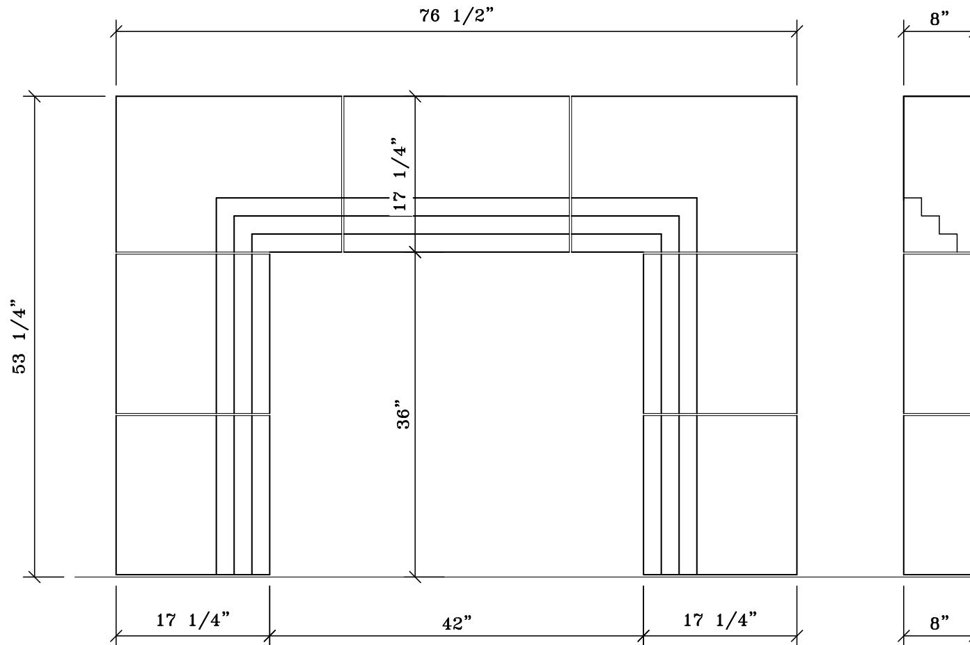
FRONT VIEW
