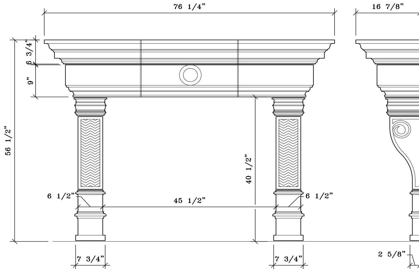
FRONT VIEW
